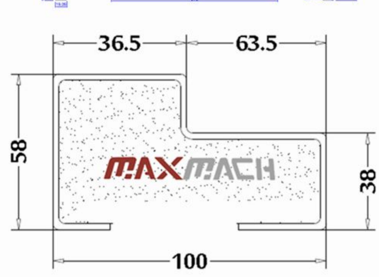
100 X 58 mm REBATE PROFILE
