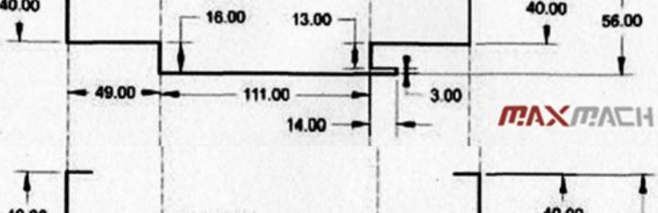
100 X 70 mm REBATE PROFILE
