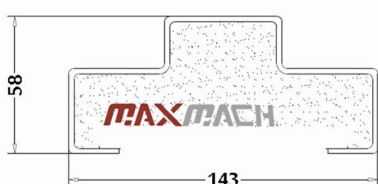
143X 58 mm REBATE PROFILE
