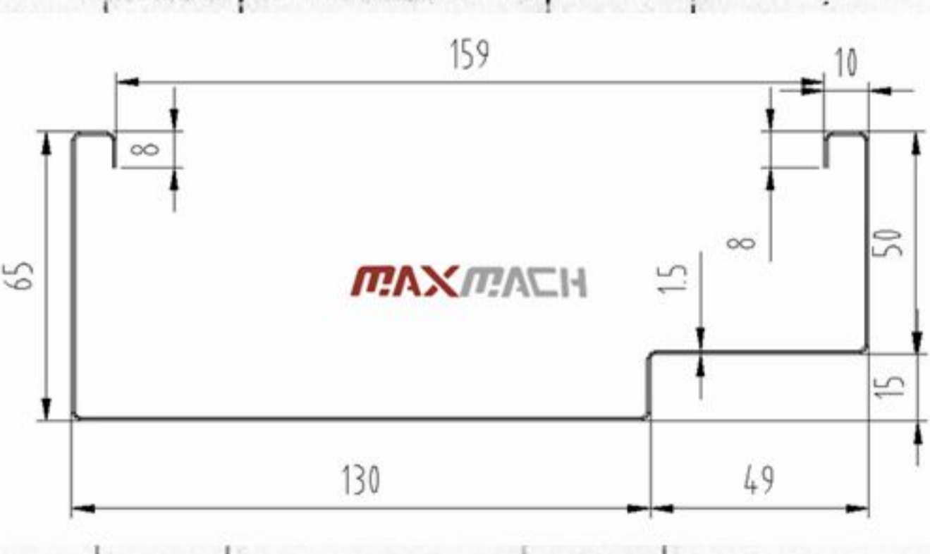
130 X 70 mm REBATE PROFILE
